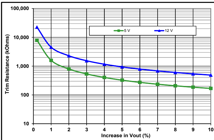
Common Figure 3: Trim-Up Graph for 5 to 12V outputs.
