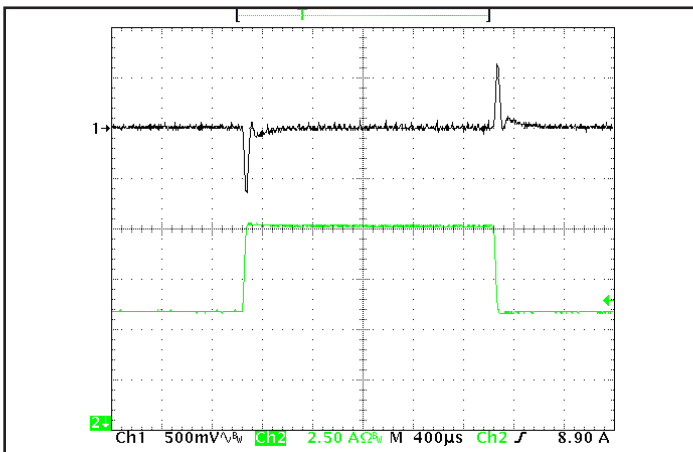
Figure 5: Output voltage response to step-change in load current (50% -75% -50% of I out (max); dI/dt = 0.1 A/μs. Load cap: 15 μF tantalum cap and 1 μF ceramic cap. Ch 1: V out , Ch 2: I out (2.5 A/div).
